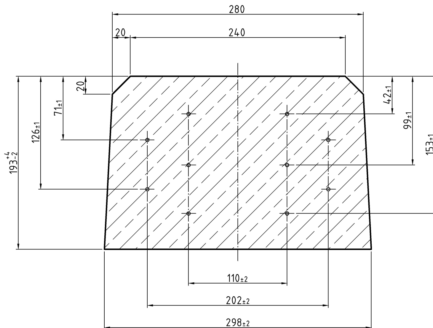
A - A 1:2.5
